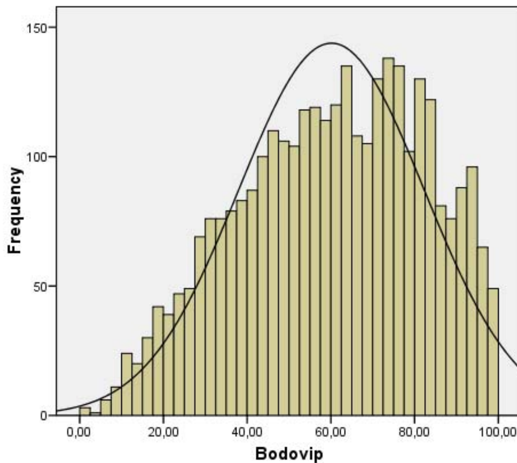
Histogram
