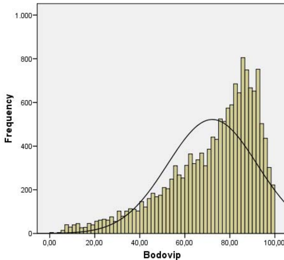
Histogram
